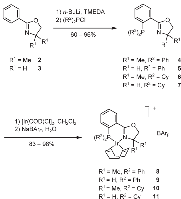
Scheme 1. Synthesis of Ir-PHOX complexes 8–11 .
