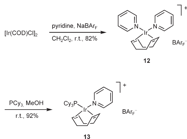
Scheme 2. Synthesis of iridium complex 13 .
